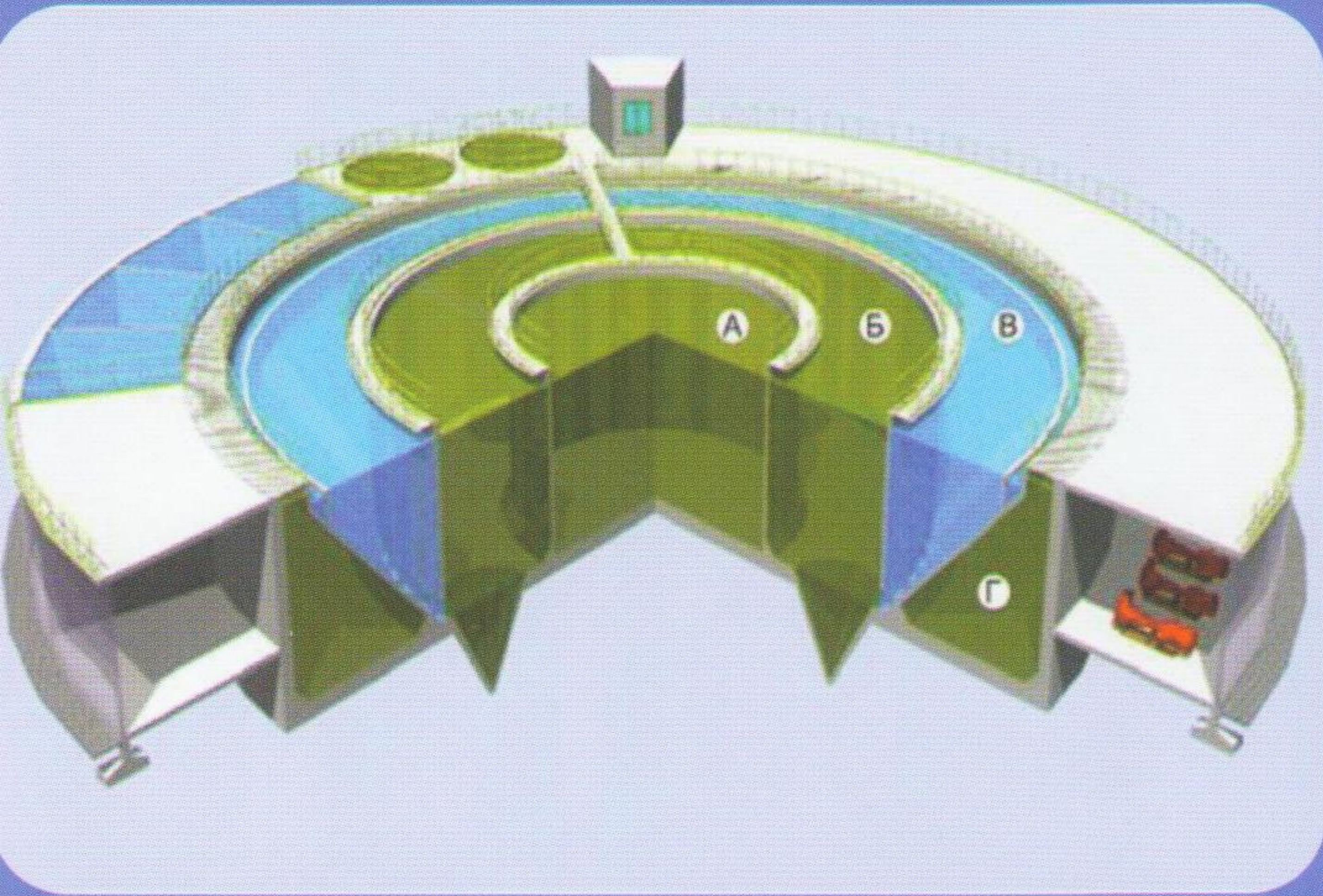
Modular station for deep municipal sewage treatment
