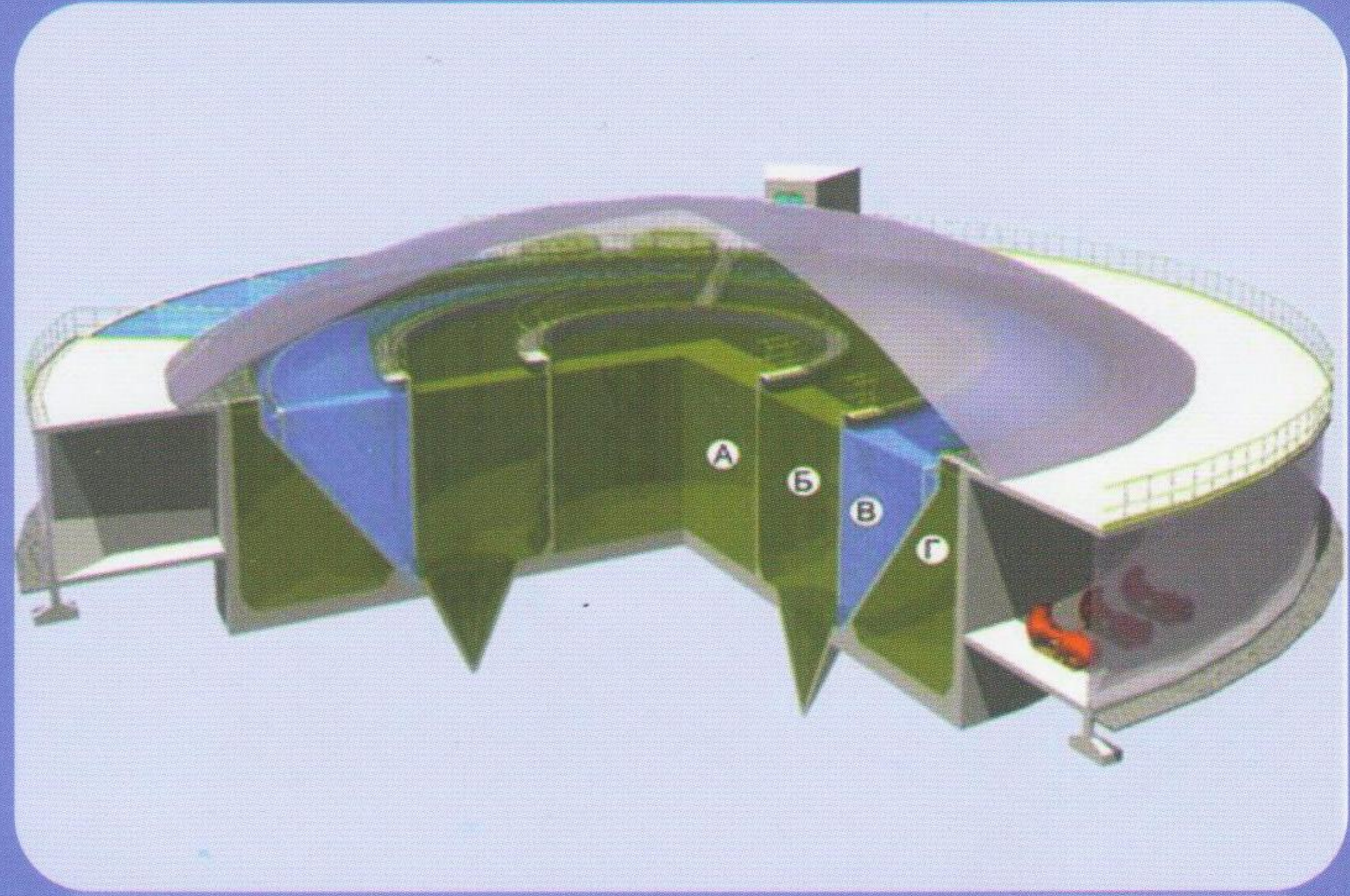
Treatment station variant: Closed-type building
